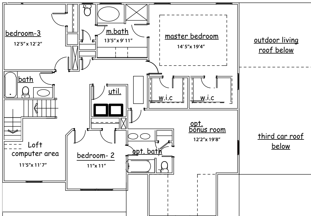
Second Floor-1676 SQ FT
