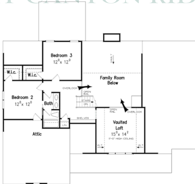
SECOND FLOOR 799sf
