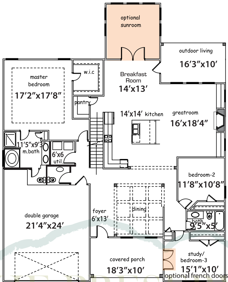
Main Floor-2264 SQ FT
