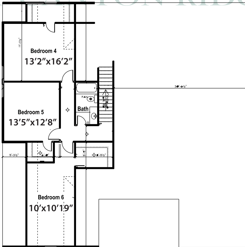
2nd Floor-978 SQ FT
